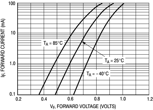
Figure 3. Forward Voltage
