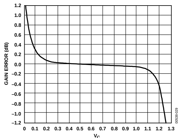
Figure 31. Gain Error for Cascaded Stages—Low Ripple Mode
