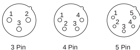
Contact Arrangement
