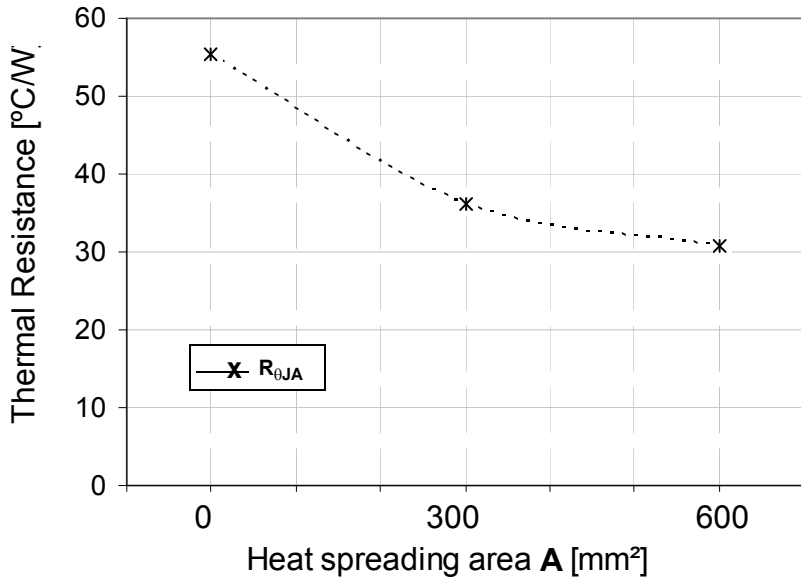
Figure 27. Device on Thermal Test Board R_{\theta\text{JA}}
