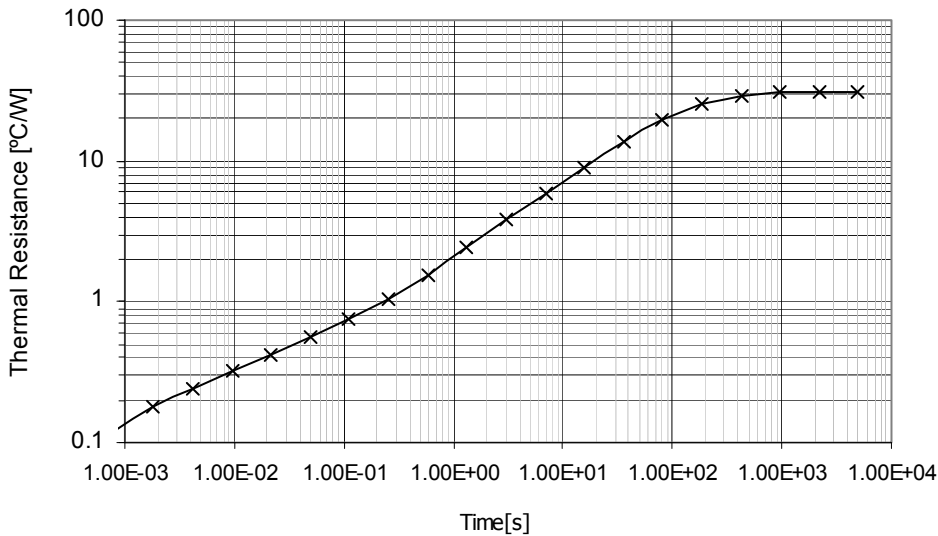
Figure 28. Transient Thermal Resistance R_{\theta\text{JA}} Device on Thermal Test Board Area A = 600 ( \text{mm}^2 )
