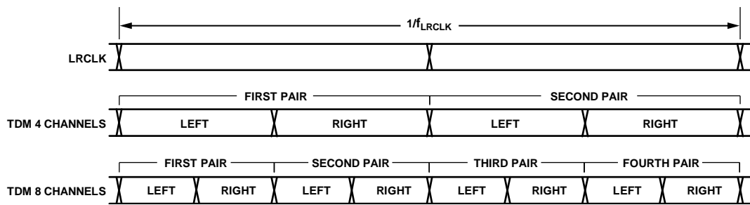
Figure 63. Left First Channel Selection in TDM
