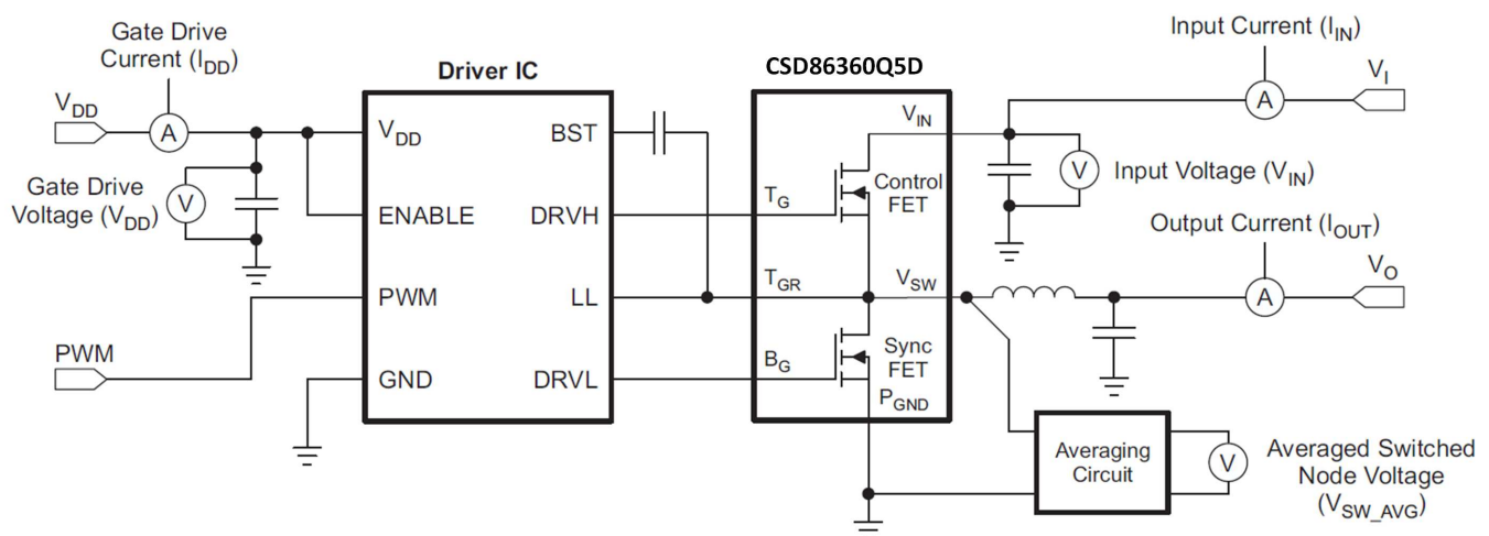
Figure 32. Typical Application
