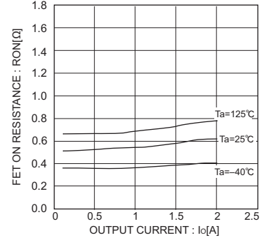
Fig.15 ON resistance VIN=7V (BD9001F)
