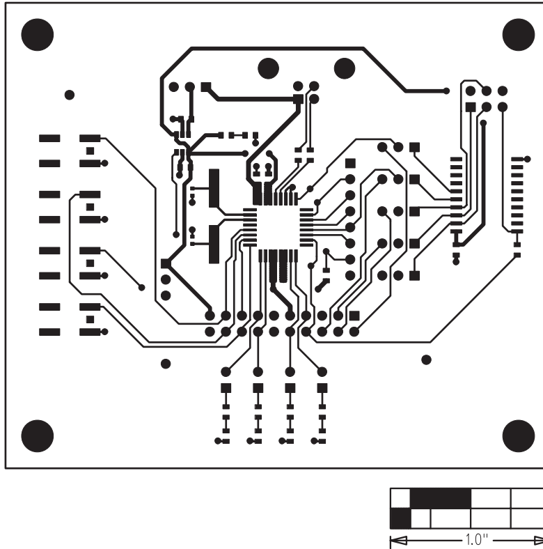
Figure 5. MAX3420E EV Kit-2 PCB Layout—Component Side
