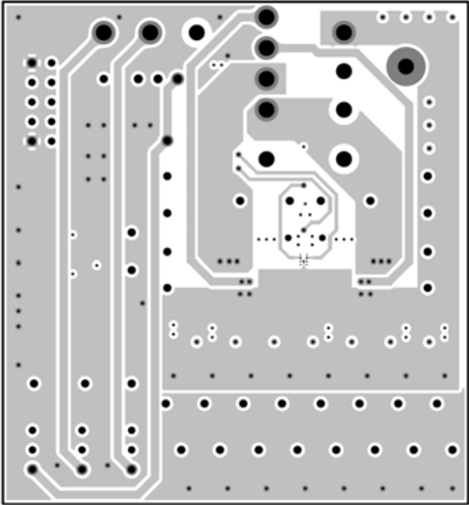
Figure 15. Layer 3 ( Top View )
