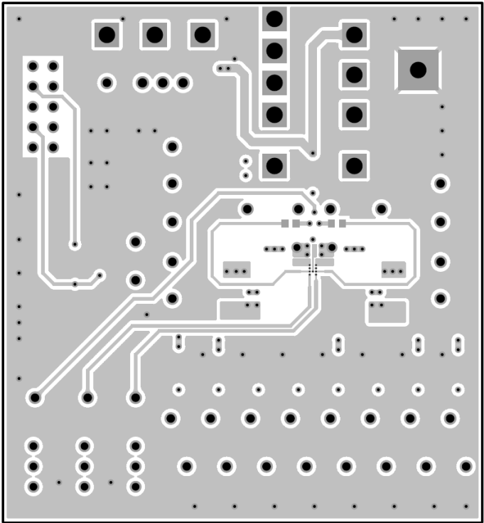
Figure 16. Bottom Layer ( Top View )
