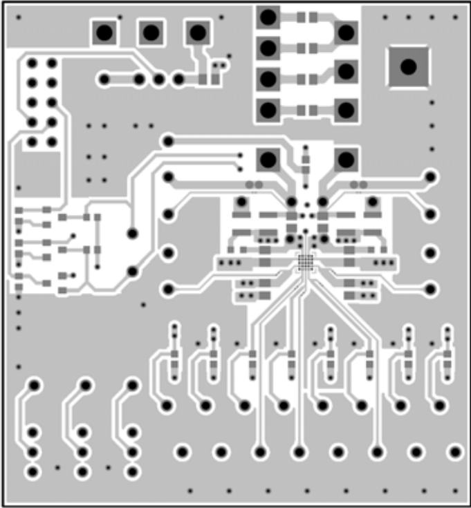
Figure 13. Top Layer ( Top View )
