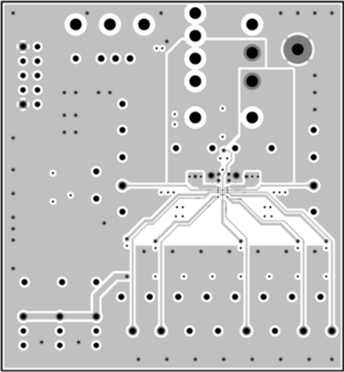
Figure 14. Layer 2 ( Top View )
