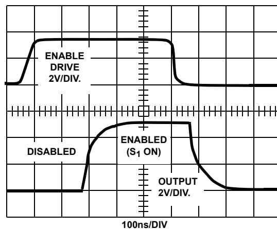
FIGURE 7C. WAVEFORMS
