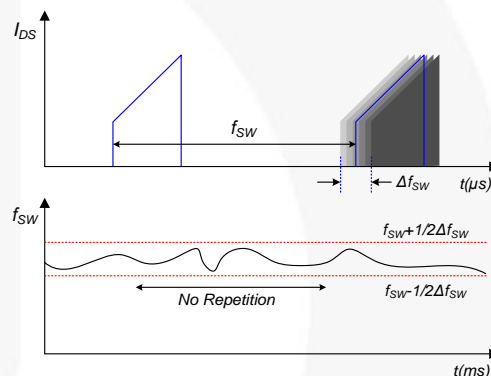
Figure 26. Random Frequency Fluctuation
