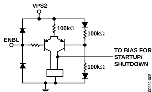
Figure 25. Circuit C
