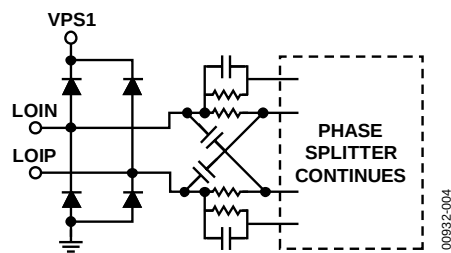
Figure 24. Circuit B
