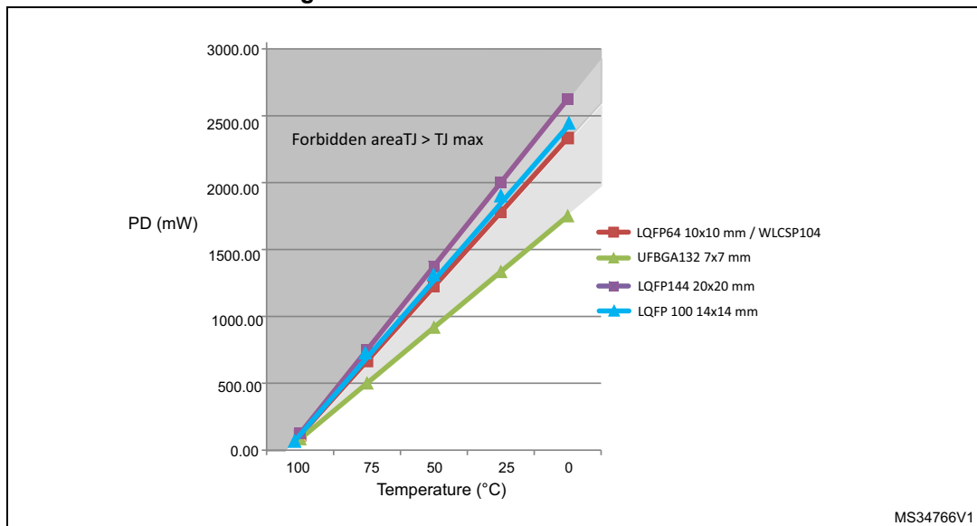
Figure 46. Thermal resistance suffix 6
