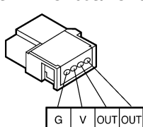
SRT2-VOD08S/VOD08S-1
