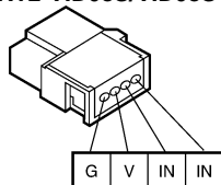
SRT2-VID08S/VID08S-1
