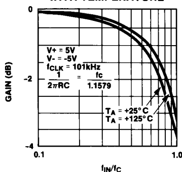
VARIAION OF PASSBAND GAIN WITH TEMPERATURE
