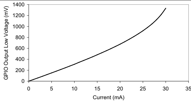
Figure 4-17. GPIO Output Low Voltage vs Current Being Sunk
