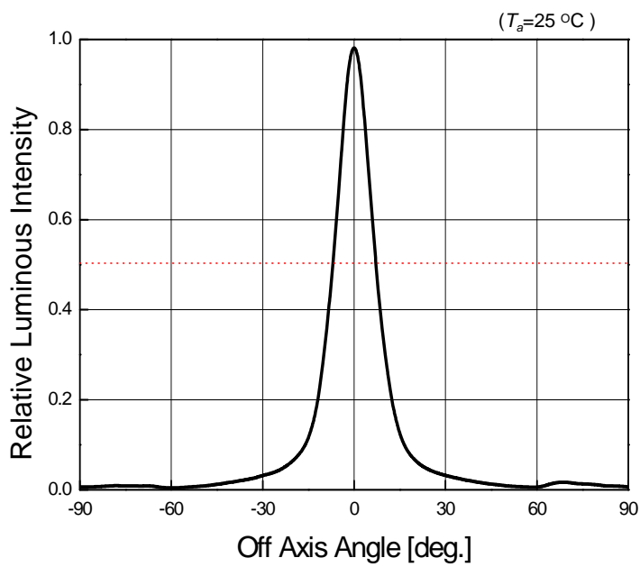
Radiation Diagram
