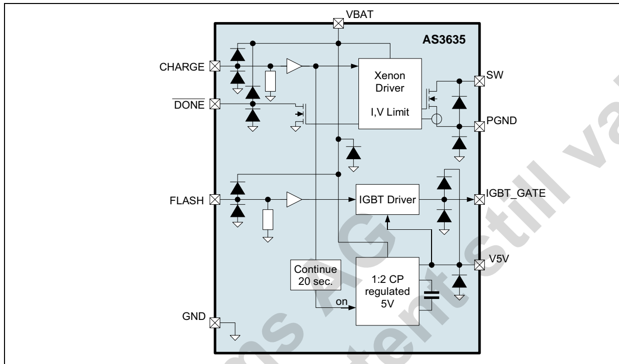
Figure 21. ESD Diodes
