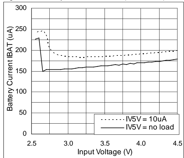
Figure 14. Battery current vs. VBAT (V5V CP on)
