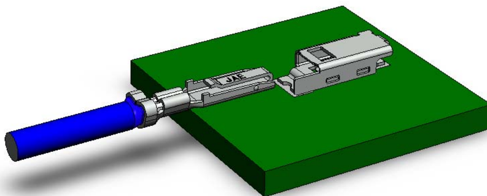
Socket (ES5S001JF1) Plug (ES5P09K5F1)
