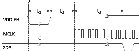
Figure 1 Power-Up Sequence
