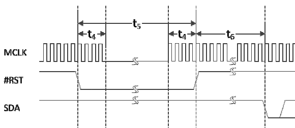
Figure 2 Reset Sequence
