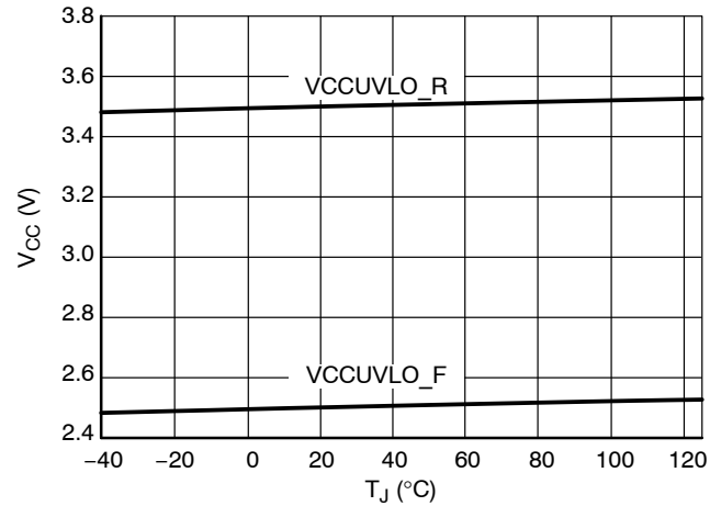
Figure 6. V CCUVLO
