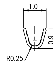
WIRE BARREL
