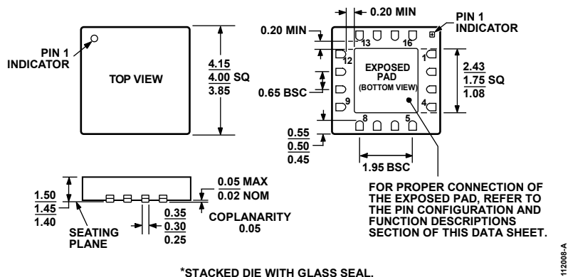
*STACKED DIE WITH GLASS SEAL. Figure 27. 16-Lead Lead Frame Chip Scale Package [LFCSP_LQ] 4 mm × 4 mm Body, 1.45 mm Thick Quad (CP-16-5a*) Dimensions shown in millimeters
