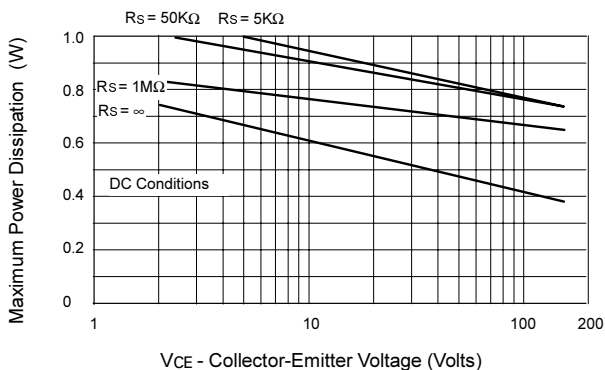
Voltage Derating Graph
