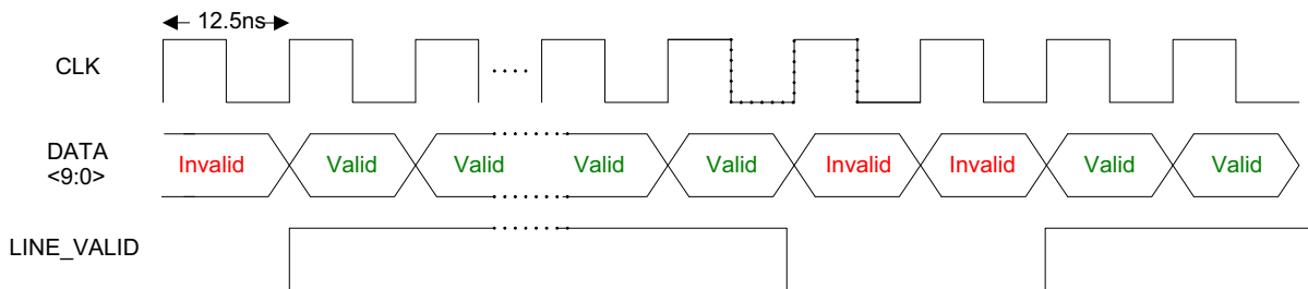
Figure 20. LINE_VALID Timing
