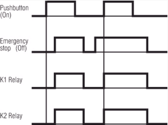
Function diagram
