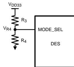
Figure 19. MODE_SEL Connection Diagram
