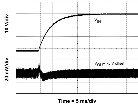
Figure 37. Line Transient (8 V to 40 V)
