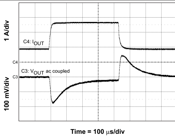
Figure 36. Load Transient
