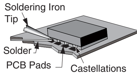
Figure 47: Soldering Technique
