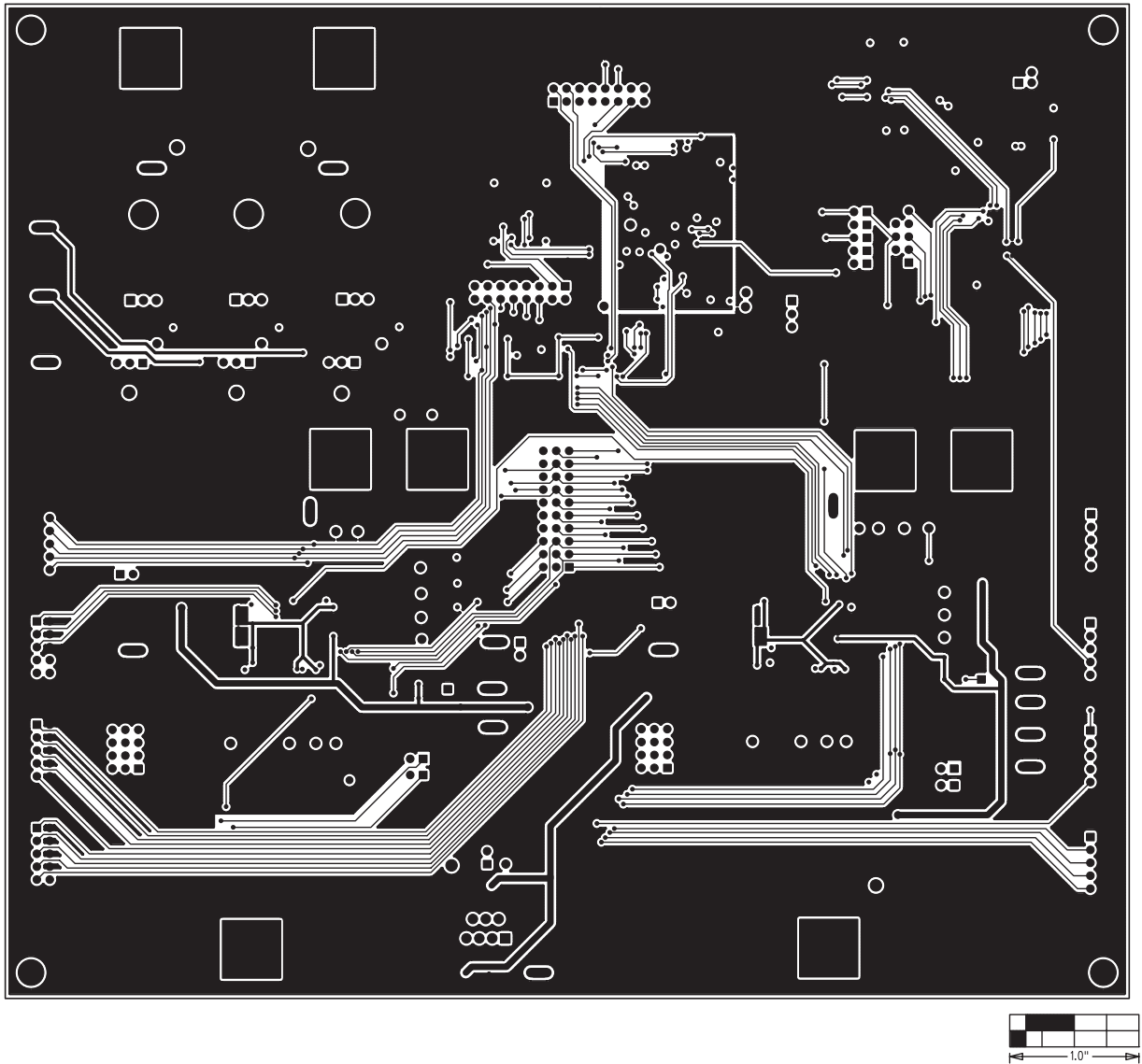
Figure 8. MAX9959 EV Kit PCB Layout—Solder Side
