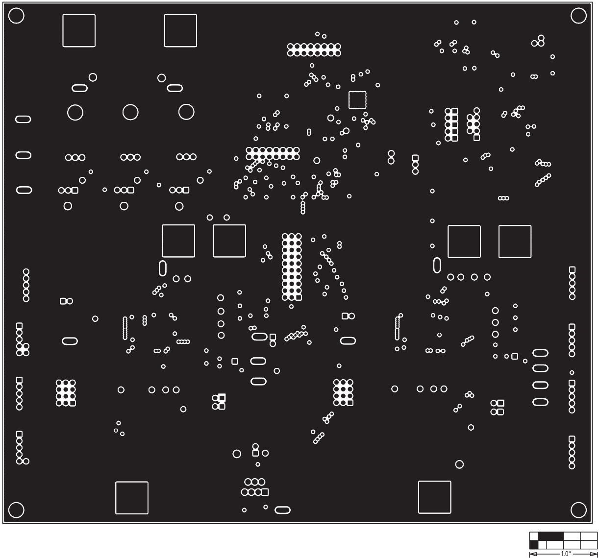
Figure 6. MAX9959 EV Kit PCB Layout—2nd Layer
