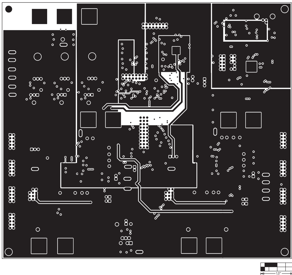
Figure 7. MAX9959 EV Kit PCB Layout—3rd Layer
