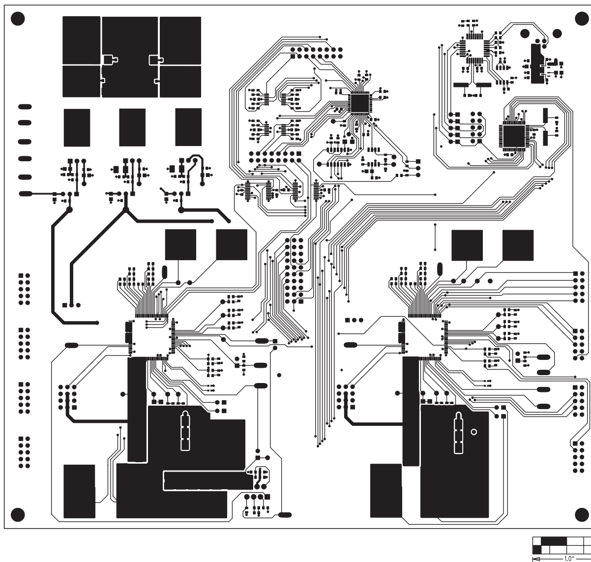
Figure 5. MAX9959 EV Kit PCB Layout—Component Side
