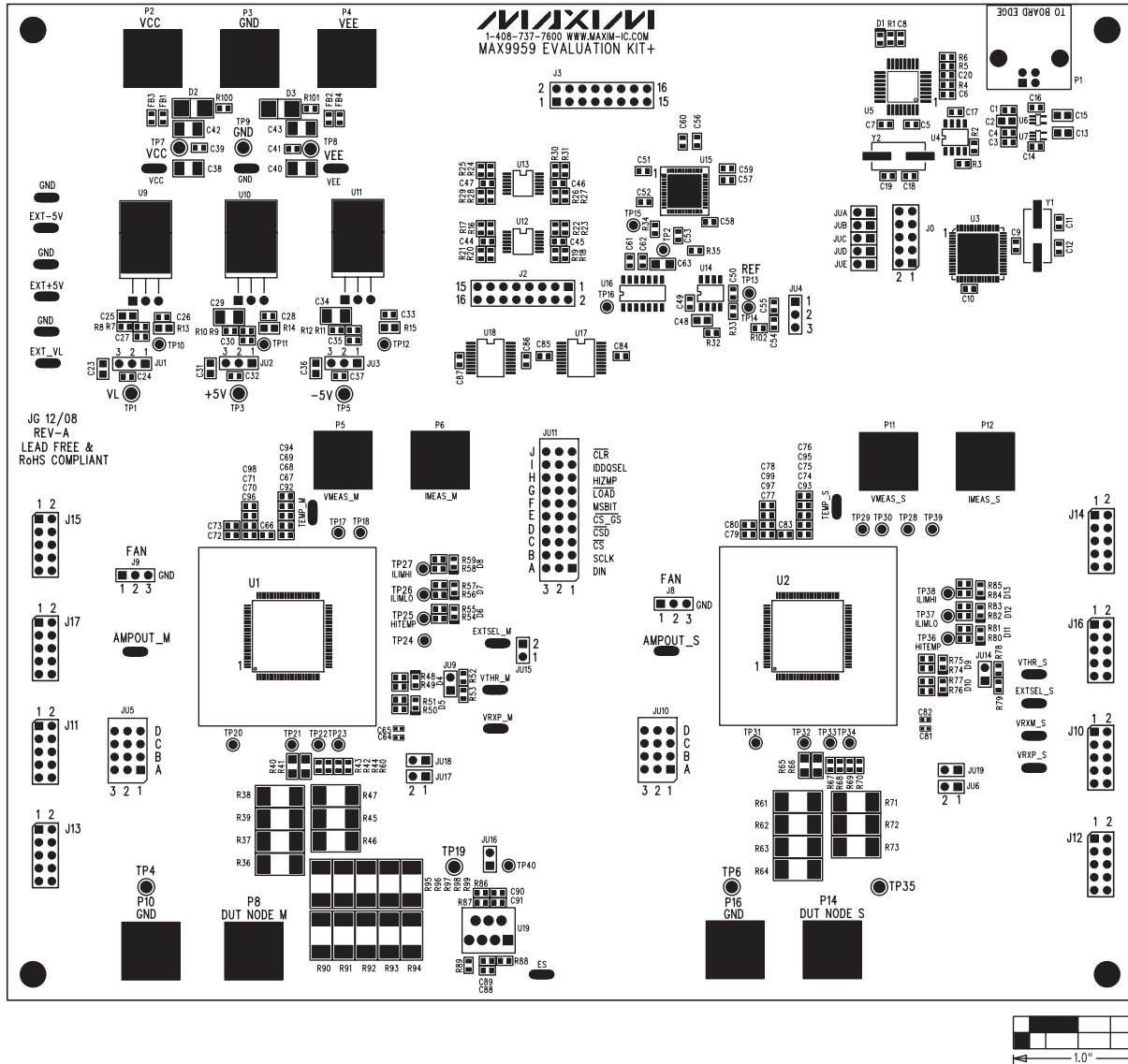
Figure 4. MAX9959 EV Kit Component Placement Guide—Component Side
