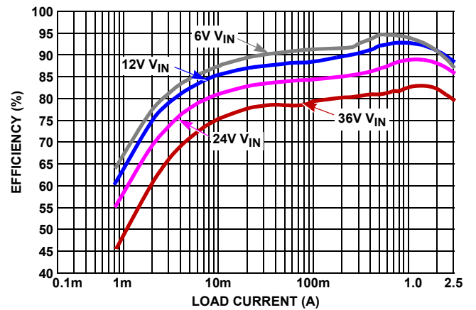
FIGURE 8. EFFICIENCY, SYNCHRONOUS BUCK, PFM MODE, V_{OUT} 3.3V, T_A = +25^\circ\text{C}
