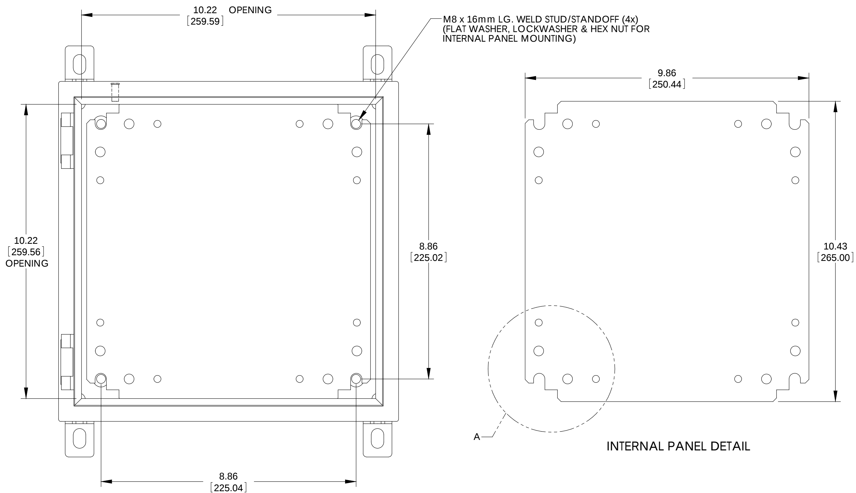
FRONT VIEW (LESS COVER)
