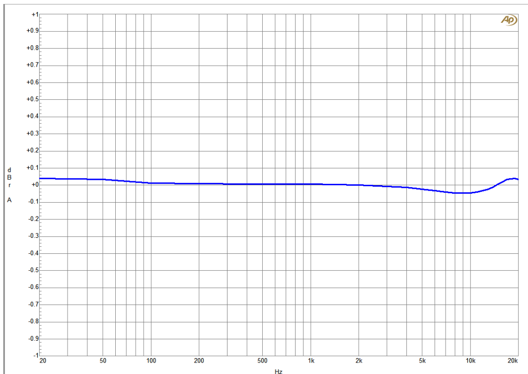
Figure 2. WM8523 Frequency Response (0 dB FS)
