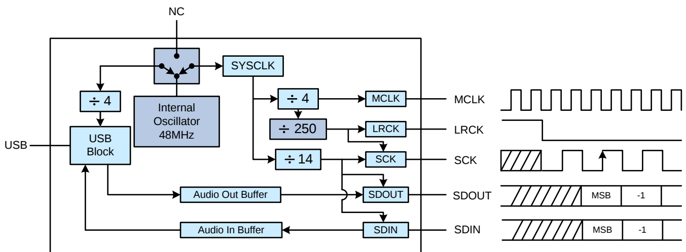
Figure 11. Configuration 1 Example
