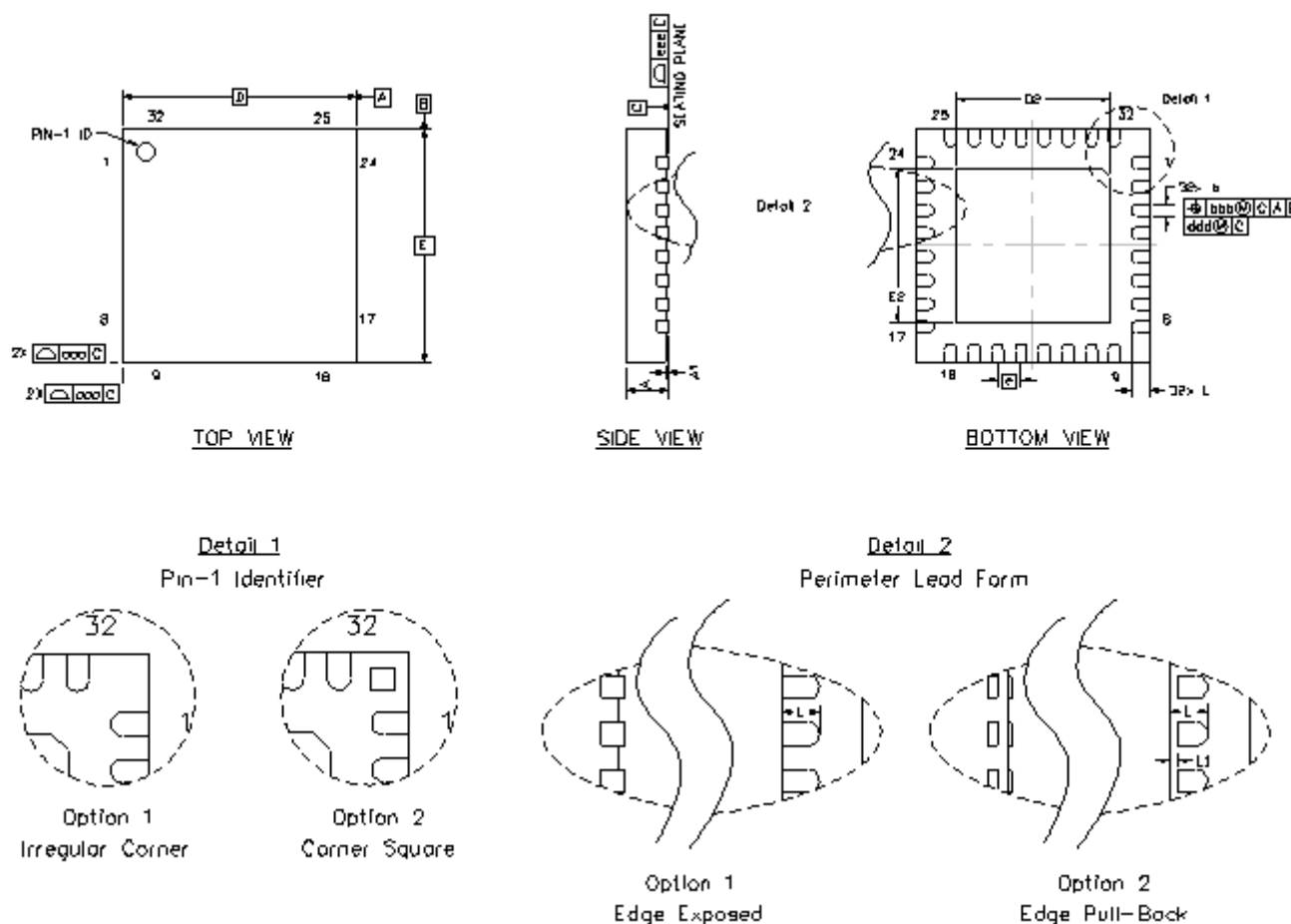
Figure 6. QFN-32 Package Drawing
