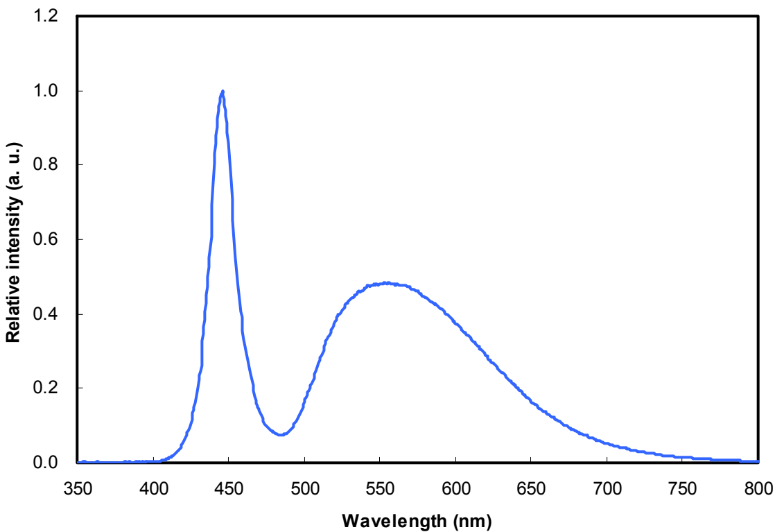
Wavelength Characteristics T_a = 25^{\circ}\text{C}
