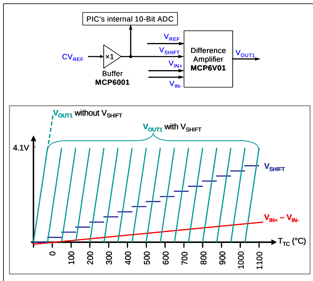
FIGURE 1-4: V_{SHIFT} Operation Conceptual Diagram.
