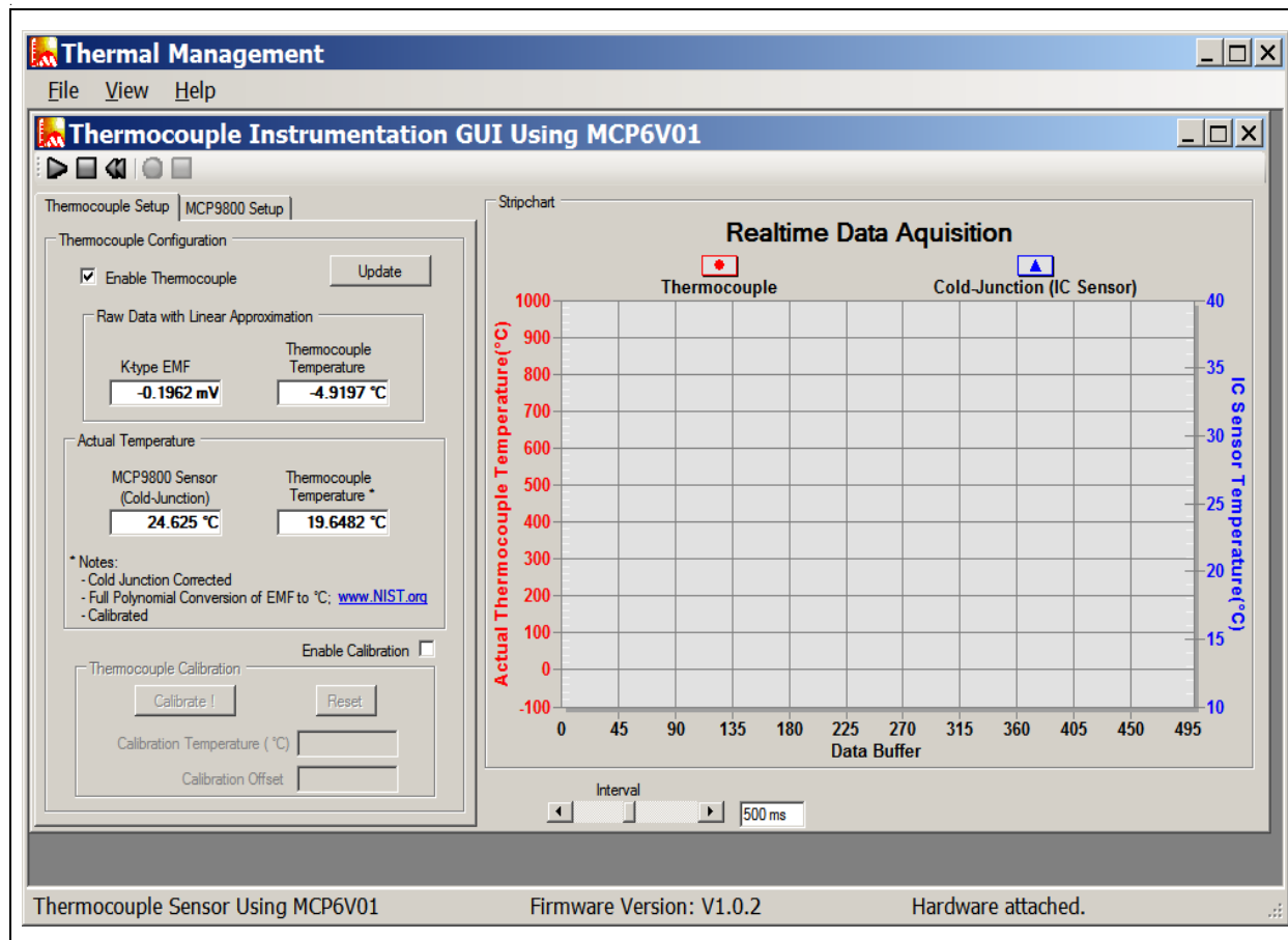
FIGURE 2-5: Thermocouple setup.
