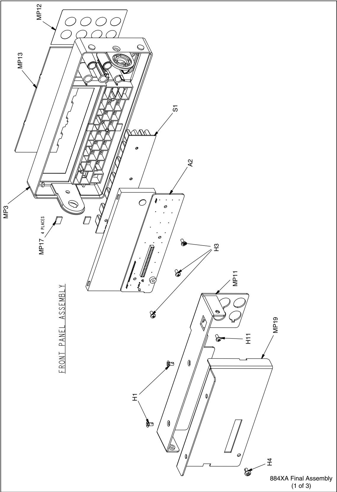
Figure 4-1. Final Assembly
