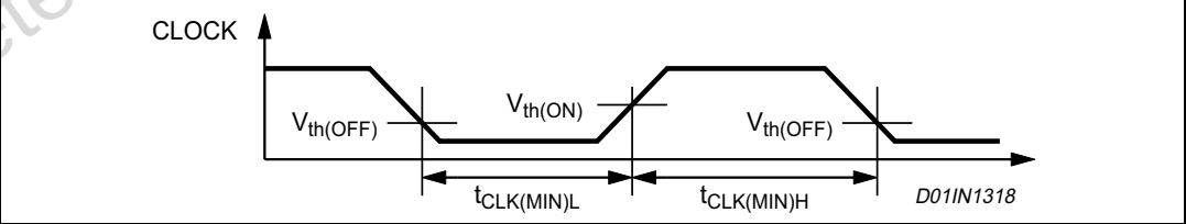
Figure 5. Minimum timing definition: clock
