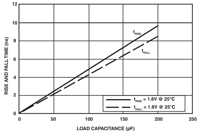
Figure 57. Driver Type A Typical Rise and Fall Times (10%–90%) vs. Load Capacitance (1.8V V_{DDEXT}/V_{DDMEM} )
