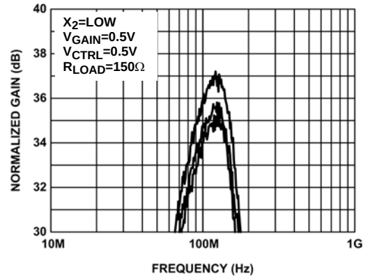
FIGURE 6. CHANNEL MISMATCH
