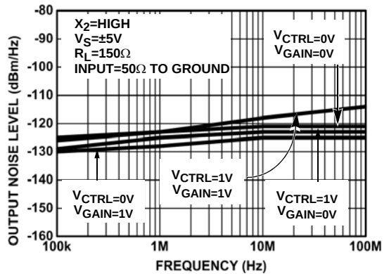
FIGURE 10. OUTPUT NOISE
