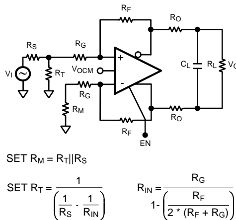
Figure 32. Single Ended in Differential Out
