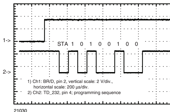
Fig. 3 - Programming sequence for setting the endec to a bit rate of 12.8 kbit/s as in figure 2 but with a 3/16 bit pulse duration (S0 = "0").
