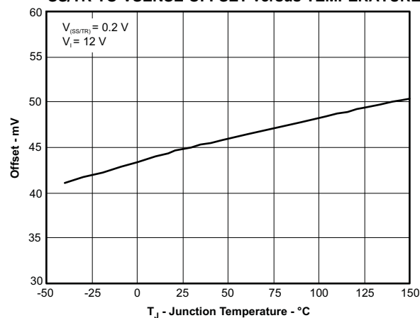
SS/TR TO VSENSE OFFSET versus TEMPERATURE
