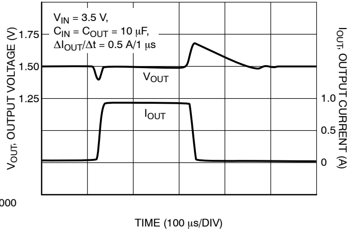
Figure 22. Load Transient ( V_{out} = 1.5 \text{ V} )
