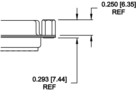
03X..... 0.250" (MATING SIDE) - CN8
