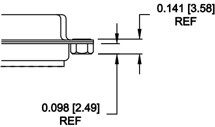
01X ..... 0.098" (BOARD SIDE) - CN1
