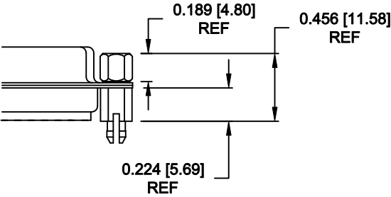
91X ..... 0.224" BOARD SIDE 0.189 MATING SIDE CN10/SF504404
