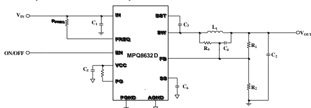
Figure 55—Schematic for PCB Layout Guide
