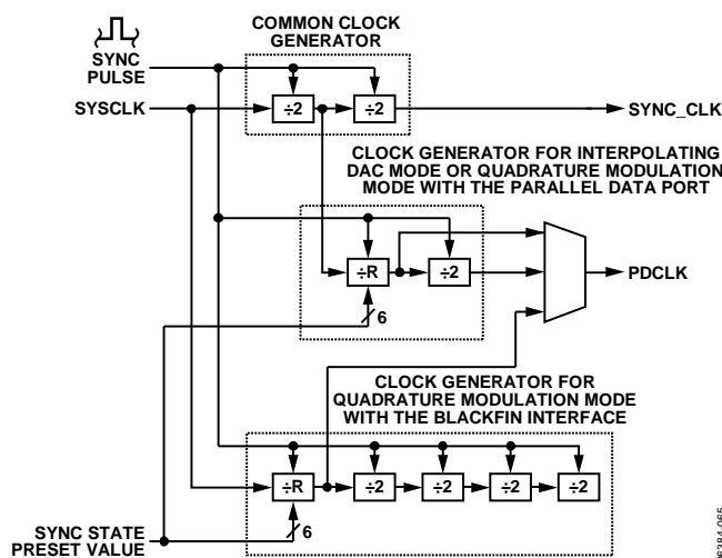
Figure 55. Clock Generator
