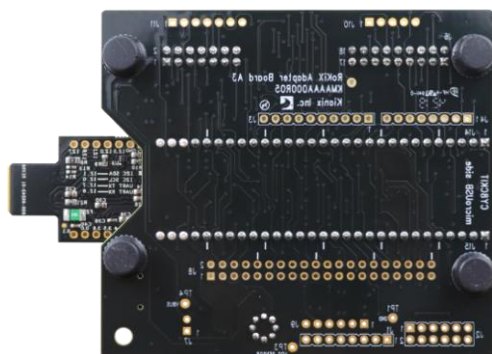
Figure 2. RKX-EVK-001 (Bottom)
