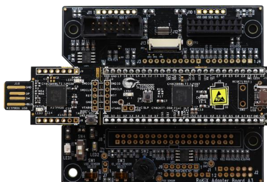
Figure 1. RKX-EVK-001 (Top)
