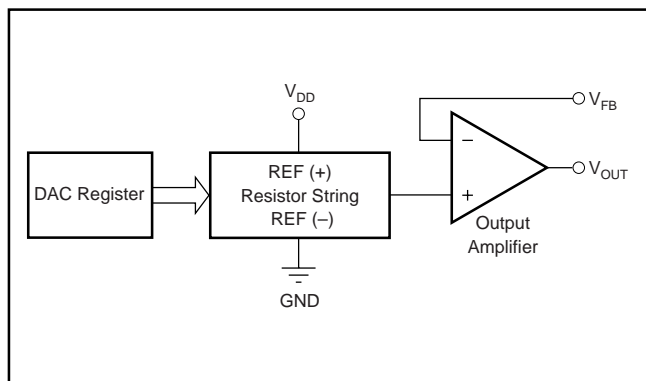
FIGURE 1. DAC7513 Architecture.
