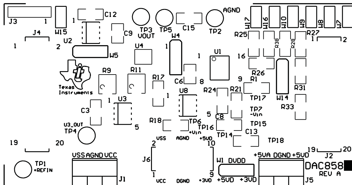
Figure 2. Top Silkscreen
