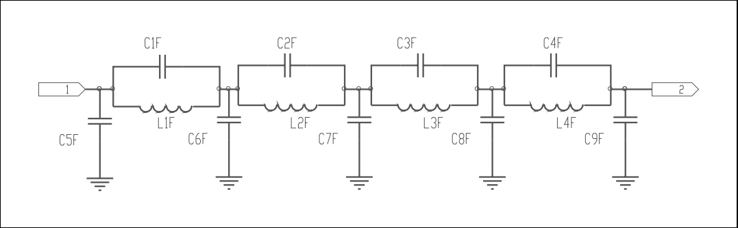
Figure 9. Filter schematic
